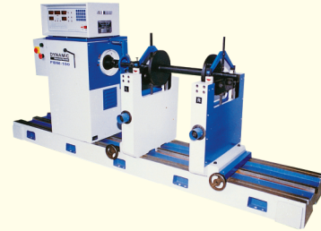
DYNAMIC BALANCING MACHINES HORIZONTAL TYPE ( Model : FBM - M )
